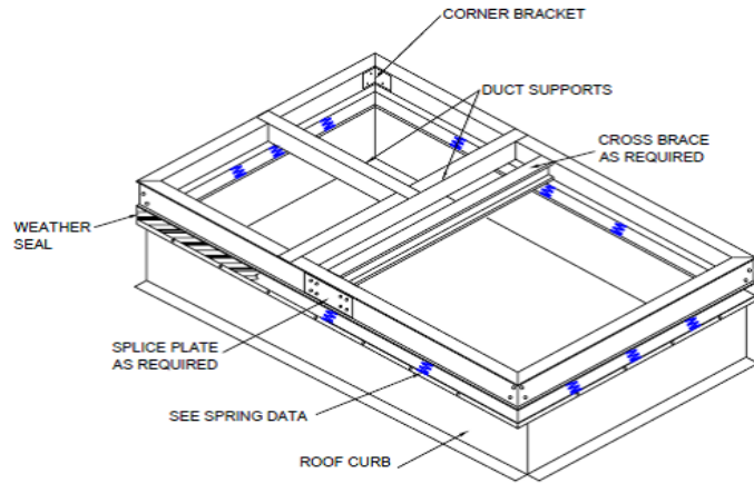
ISOMETRIC VIEW
